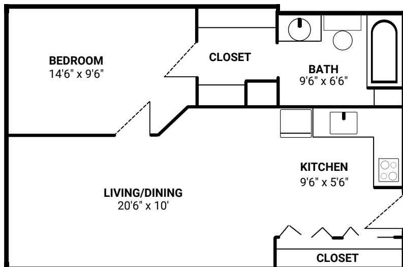
Floor Plan H - 605 sq. ft.
